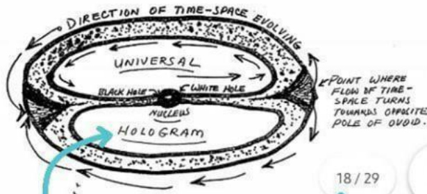
Figure B Diagram of the Cosmic Egg
