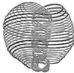
Figure C Stylized Rendition of a Simple Torus
